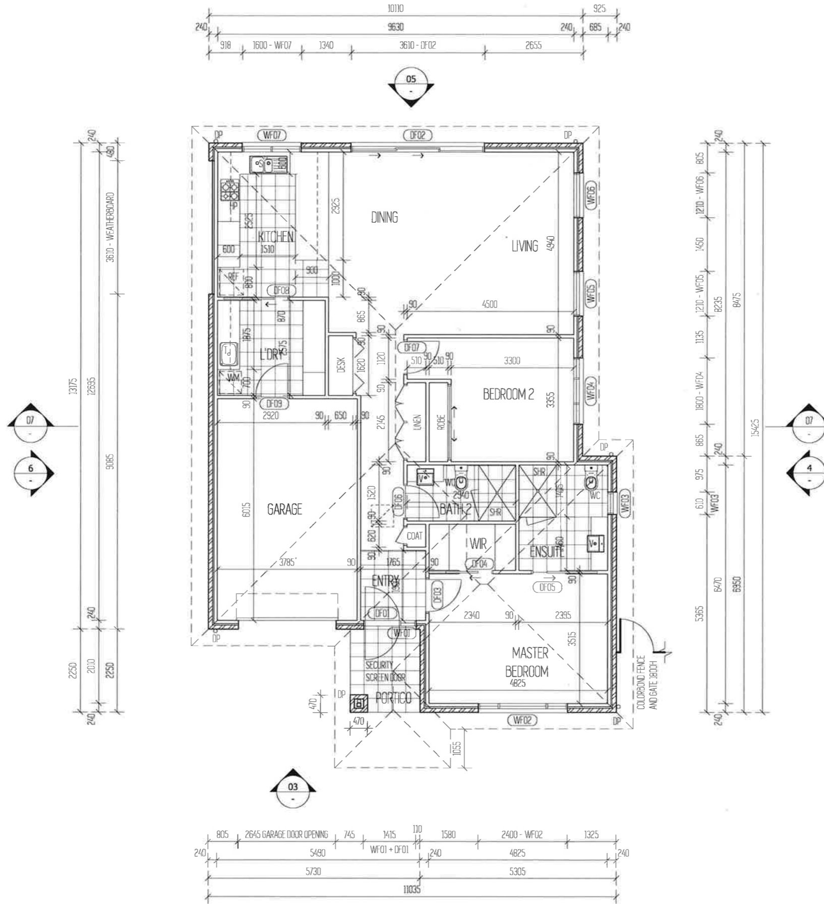
01 TYPE MARSHALL (LH STANDALONE) - FLOOR PLAN SCALE: 1:100 APPLICABLE TO UNIT 115
